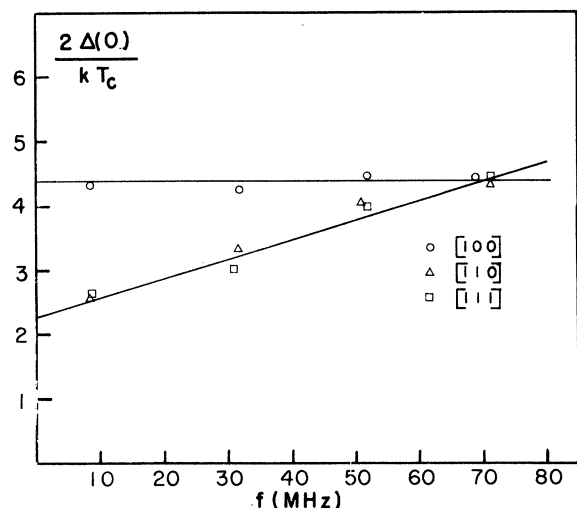
FIG. 6. Plot of 2\Delta(0)/kT_c versus the frequency f in MHz.
