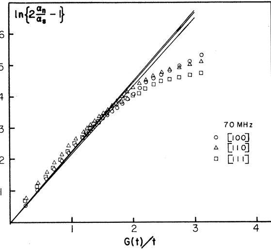
FIG. 5. Plot of \ln(2\alpha_n/\alpha_s - 1) versus G(t)/t for various directions in Pb at 70 MHz.
