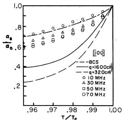
FIG. 10. Comparison of data to the calculations of Woo and the BCS theory about the transition temperature for the [100] direction in Pb.
