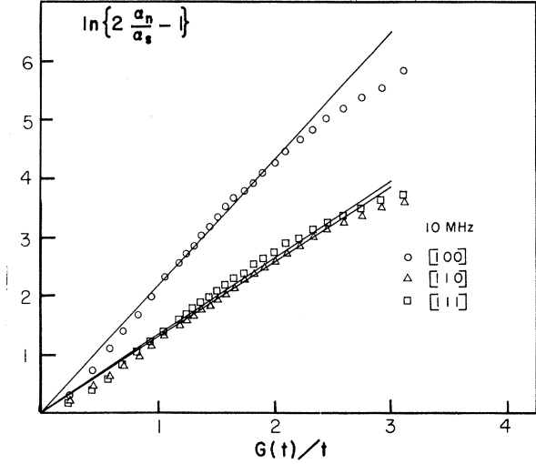
FIG. 2. Plot of \ln\{2\alpha_n/\alpha_s - 1\} versus G(t)/t for various directions in Pb at 10 MHz. The attenuations in the normal and superconducting states are \alpha_n and \alpha_s , respectively. The ratio of superconducting energy gaps is G(t) and the ratio of temperature to the transition temperature is t .
